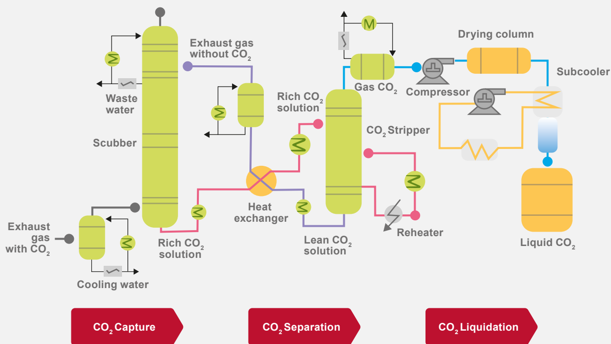
FIGURE 2.2: QIYAO ENVIRON TEC CCS SYSTEM
