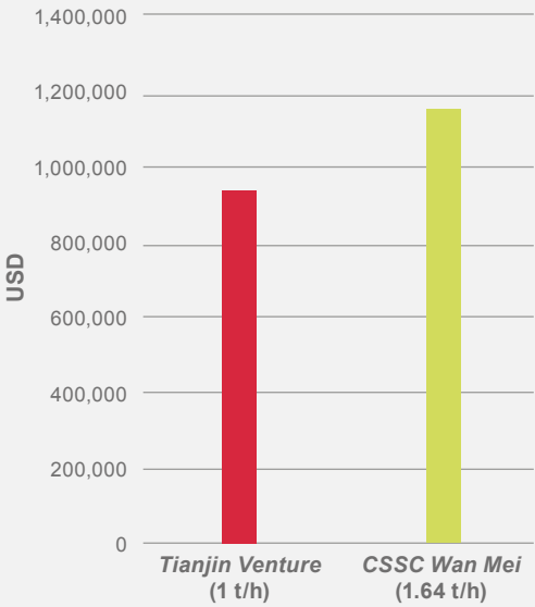
FIGURE 6.1: CAPEX OF CCS
